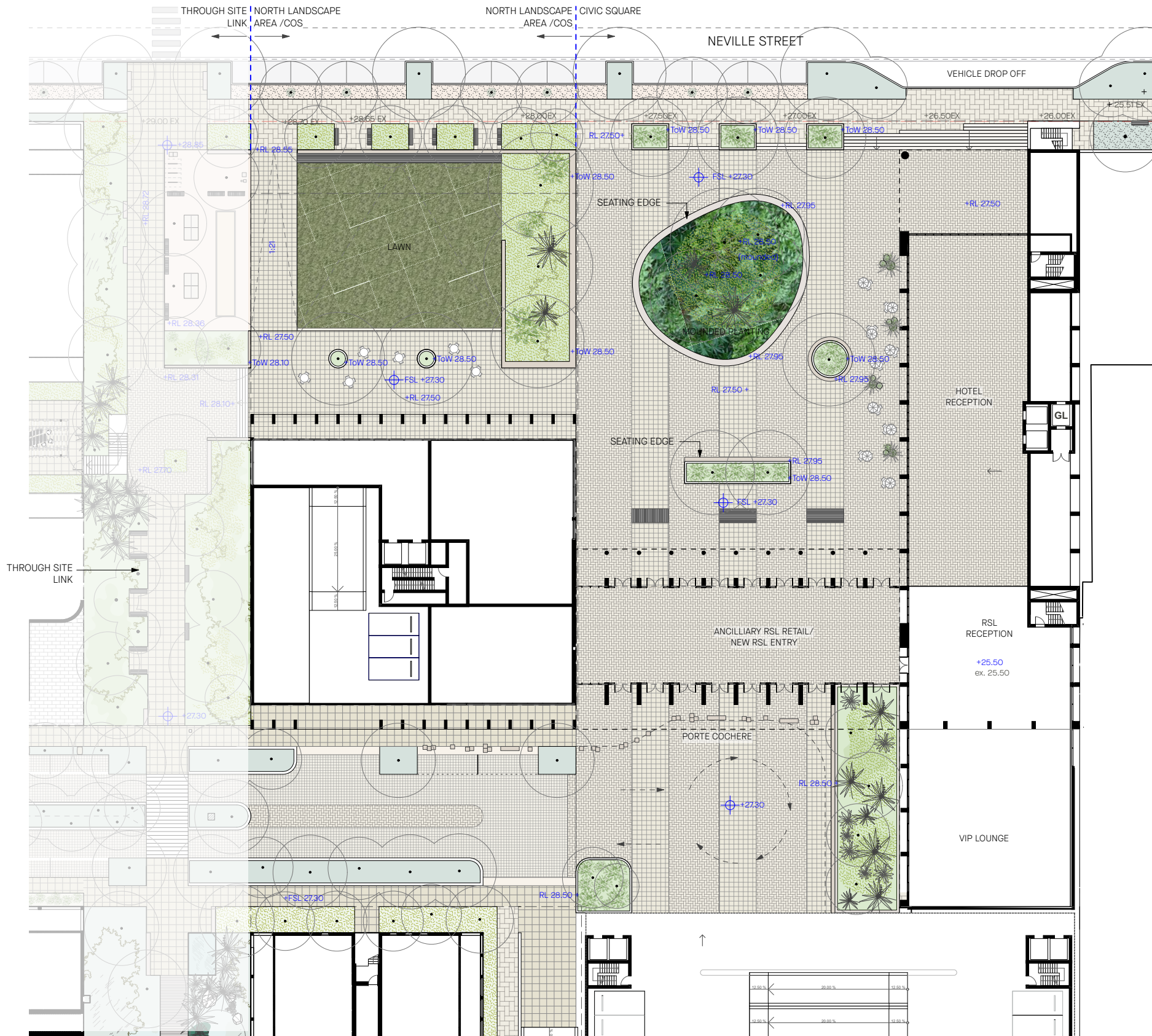
1 PLAN - CIVIC SQUARE & NORTH LANDSCAPE AREA/COS Scale: 1:500
